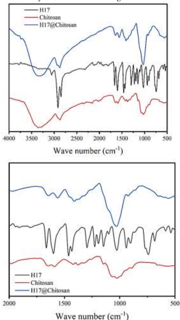
Figure 3: ATR-IR spectra of H17, CH, and H17@CH hydrogel films.
