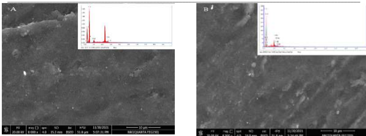
Figure 6: SEM images of (A) CH and (B) H17@CH hydrogel films and their EDS spectra.
