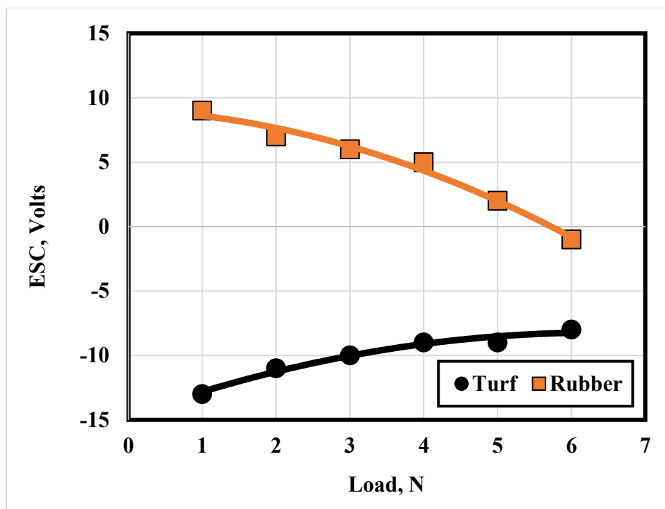
Fig. 12 Effect of applied load on ESC generated from water wet sliding of rubber on AT.
