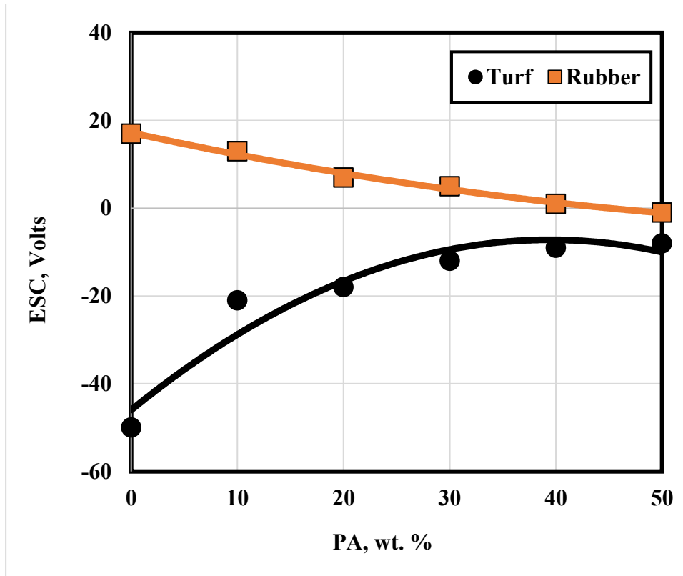
Fig. 10 ESC generated from water wet sliding of rubber on AT.
