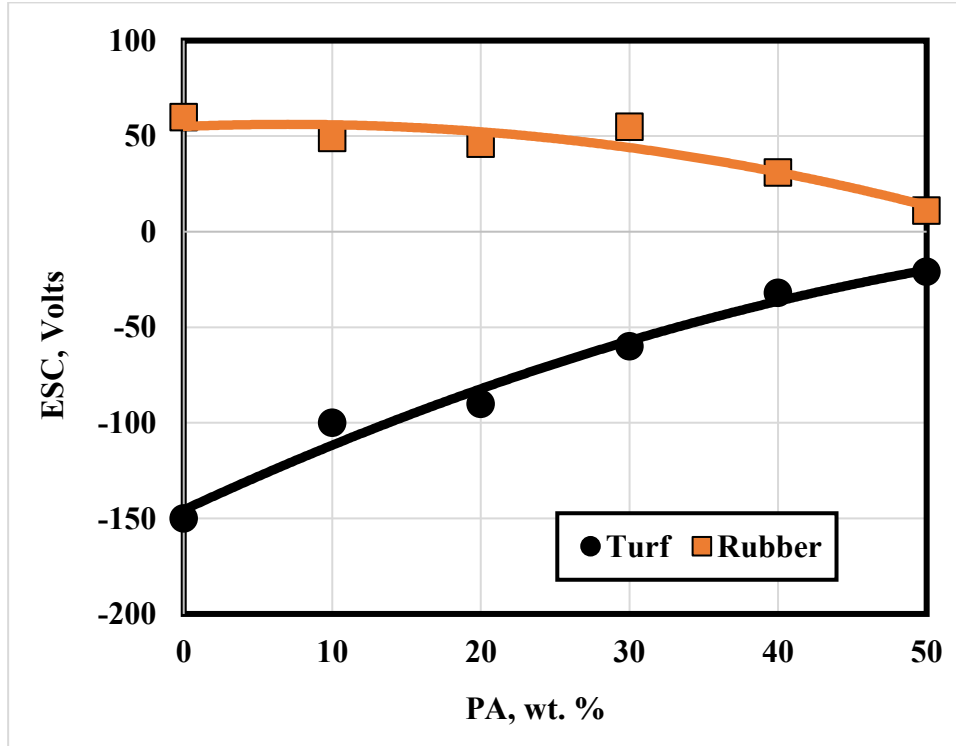
Fig. 9 ESC generated from dry sliding of rubber on AT.
