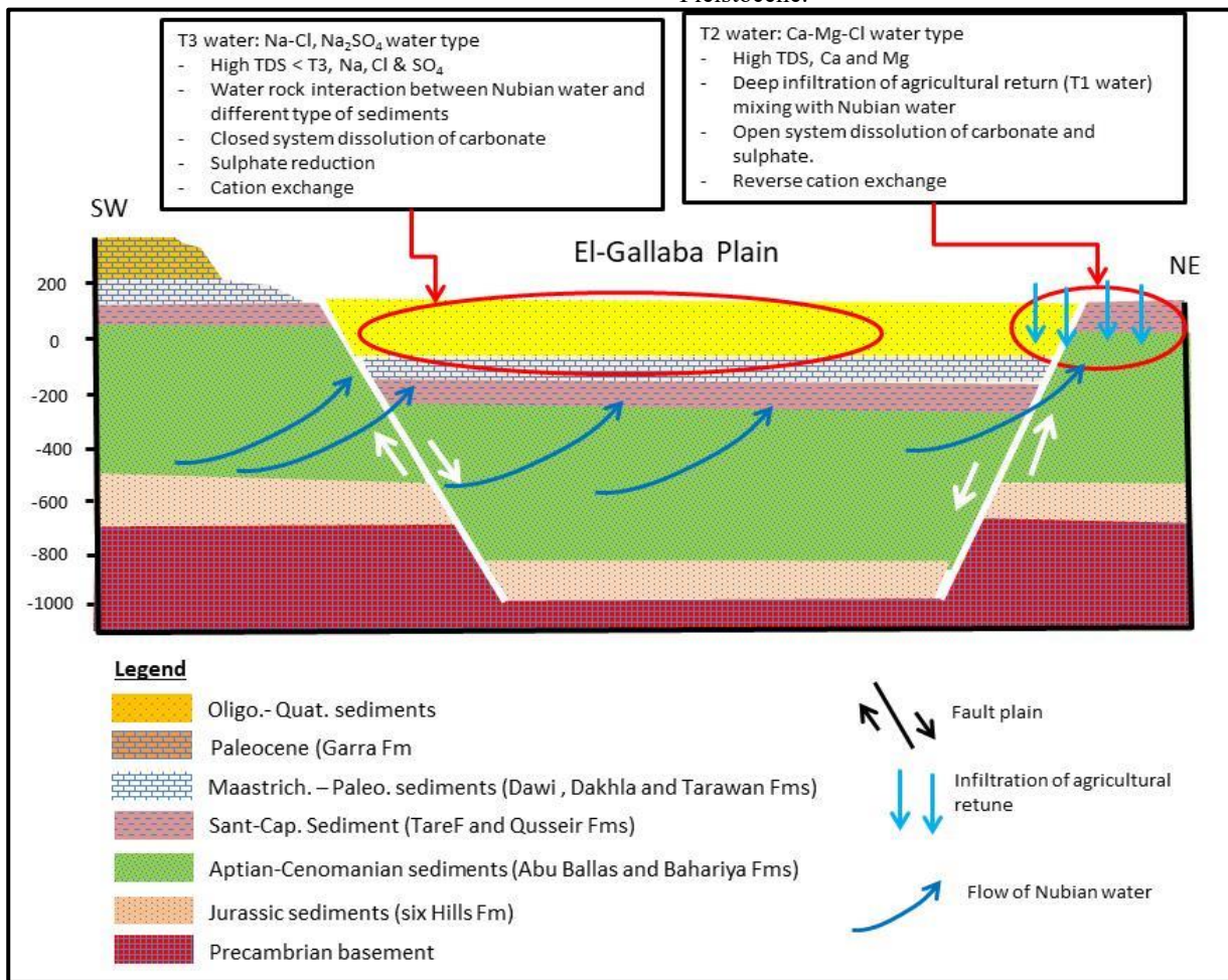
Figure 13: Schematic diagrams showing the hydrogeochemical evolution of groundwater and their controlling processes in the investigated area. Note the direction of groundwater flow from the water reservoirs in the vicinity of El Gallaba plain aquifer.
