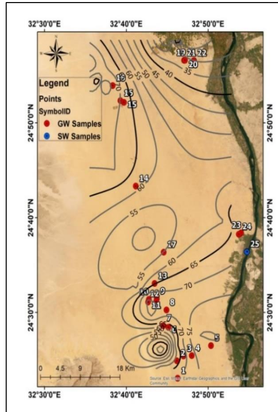
Figure 7: Groundwater level contour map of the Quaternary aquifer in El-Gallaba plain.
