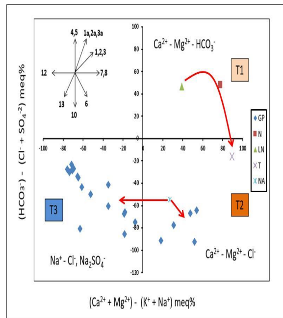
Figure 8: Geochemical classification of groundwaters; the groundwater type (T1) is Ca-Mg-HCO 3 , (T2) is Ca-Mg-Cl with MgSO 4 and MgCl 2 , and (T3) is T3 (Na-K-Cl), (Na-K-SO 4 ). The geographical locations of the groundwater types in the aquifer are shown in Figure 9. The red arrows refer to the proposed evolution trends of water types.
