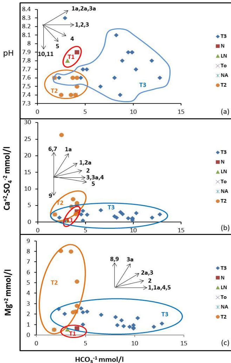
Figure10: Geochemical cross-plots of groundwaters; (a) no significant correlation between pH and \text{HCO}_3^- in T1 and T2 while the pH increased with \text{HCO}_3^- in T3, (b) relationship between (\text{Ca}^{2+} - \text{SO}_4^{2-}) and \text{HCO}_3^- ; the carbonate Ca slightly increased with \text{HCO}_3^- in T1 and T2 while no significant correlation between them in T3, and (c) Relationship between \text{Mg}^{2+} and \text{HCO}_3^- ; no significant correlation between Mg and \text{HCO}_3^- in T1 and T3 but they are significantly correlated in T2. Reaction vectors, listed in Table 2, indicate the general evolutionary geochemical trajectories of water if the indicated reaction occurs in the aquifer. Combination of reactions will lead to intermediate vectors. The vectors are not specific to any initial water type.
