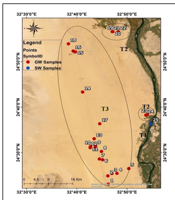
Figure 9: The geographical distribution of the groundwater types in the aquifer.
