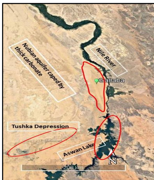
Figure 2: The Main water sources surrounding El Gallaba plain aquifer.
