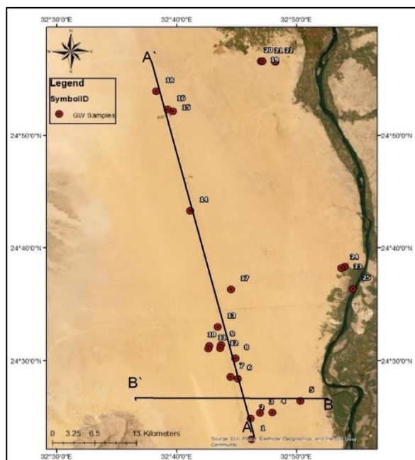
Figure 3: Locations of collected water samples.
