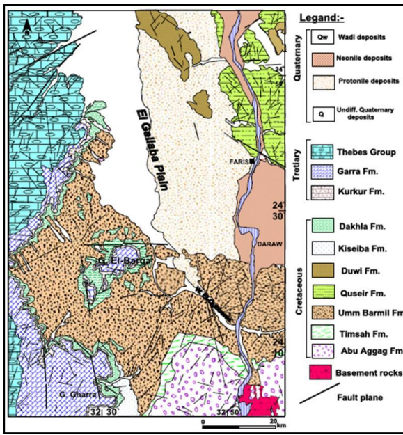
Figure 4: Geologic map of the area. Compiled after CONOCO 1987, [28], and [2].
