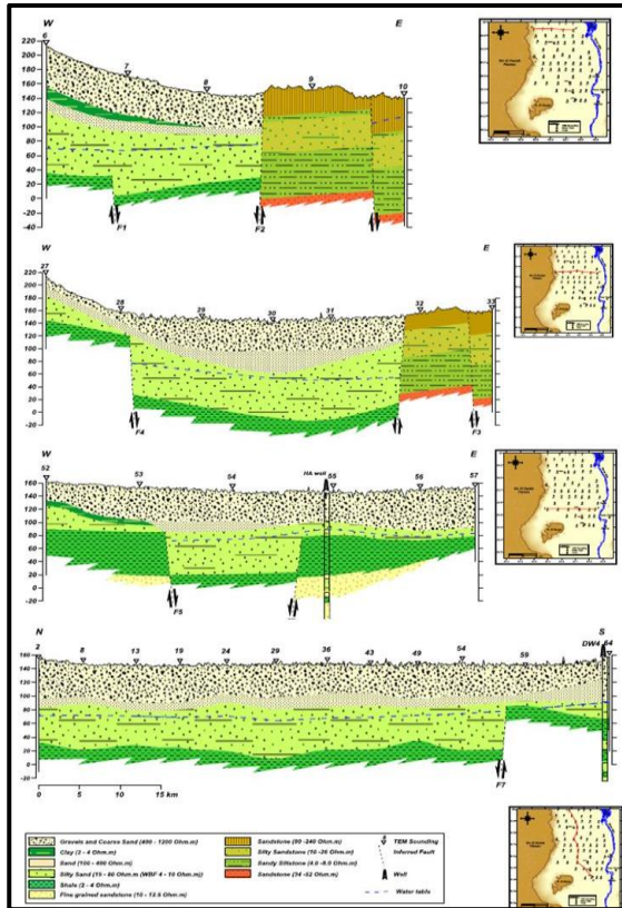
Figure 6: Geo-electromagnetic Cross-sections (Cross-sections A-A', B-B', C-C' and DD' in W-E direction Cross-section E-E' in N-S direction). [2].
