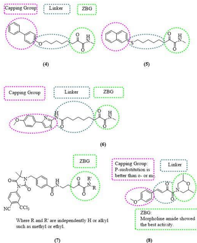
Fig. 9. Structure of compound 4, 5, 6, 7, and 8 (the \alpha -ketoamide based HDAC1s) with illustration of the main scaffolds of the structures (capping group in purple, linker in blue, and ZBG in green).
