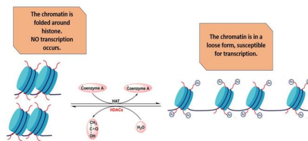
Fig. 2. Histone acetylation, deacetylation, and chromatin accessibility.
