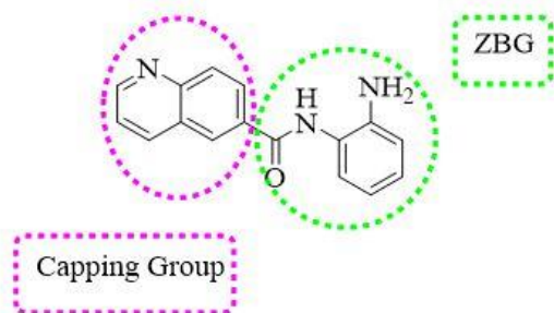
Fig. 8. Structure of the linker-less compound ( 3 ).
