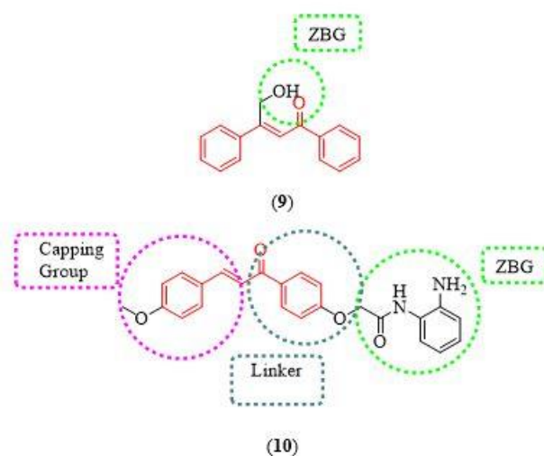
Fig. 10. Structure of compound 9 and 10 showing its main scaffold features.
