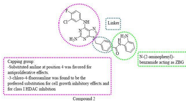
Fig. 7. Structure of MS-275, Chidamide, and compound (2) showing its main scaffold features.
