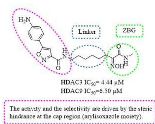
Fig. 11. Structure of compound ( 11 ) showing its main scaffold features.
