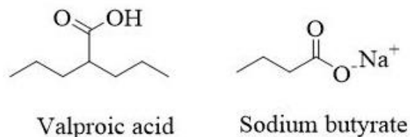
Fig. 4. Structure of short chain fatty acids HDACIs: Valproic acid and Sodium butyrate.
