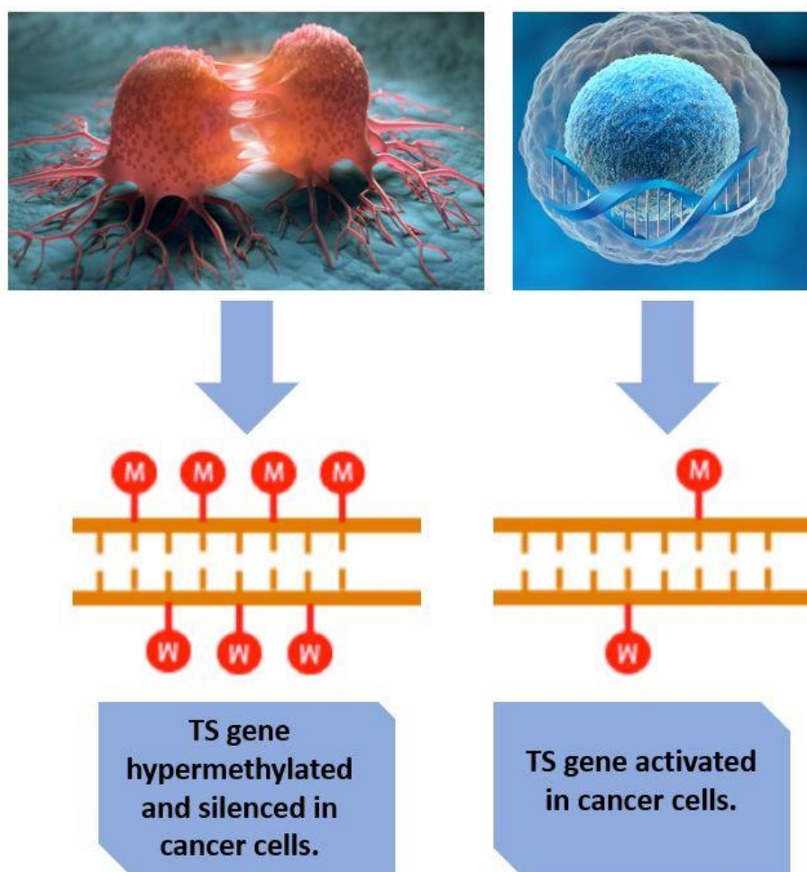
Fig. 1. Hypermethylation of TS gene in cancerous cells.
