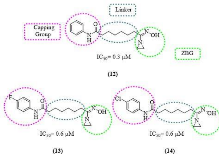
Fig. 12. Structure of compound 12 , 13 and 14 with illustration of the main scaffolds of the structures (capping group in purple, linker in blue, and ZBG in green).
