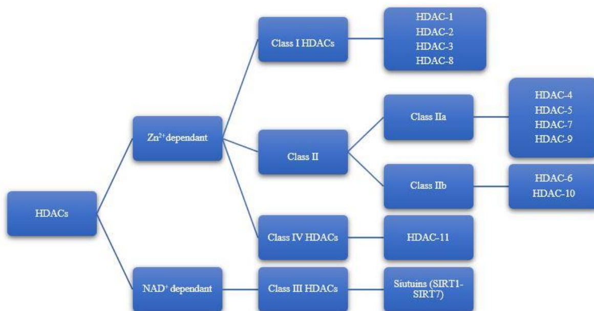
Fig. 3. HDAC isoforms classes.
