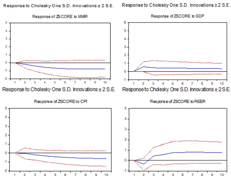
Figure 2: The impulse responses of Z-score to (MMIR, GDP, CPI, REER)
