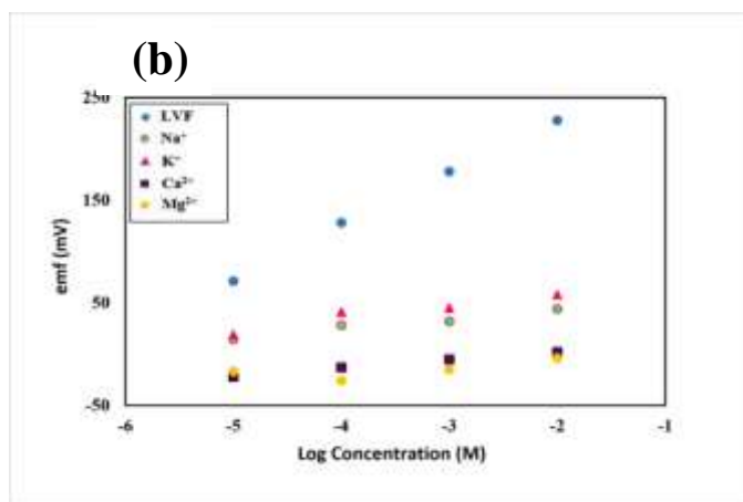
Figure 5: Calibration curves obtained for LVF and some relevant concentrations of interfering ions using (a) NIP-based electrode and (b) MIP-based electrode. The curves show a Nernstian response towards LVF due to its relative lipophilicity. Measurements were performed in ( 1 \times 10^{-2} M) acetate buffer (pH = 4.1).
