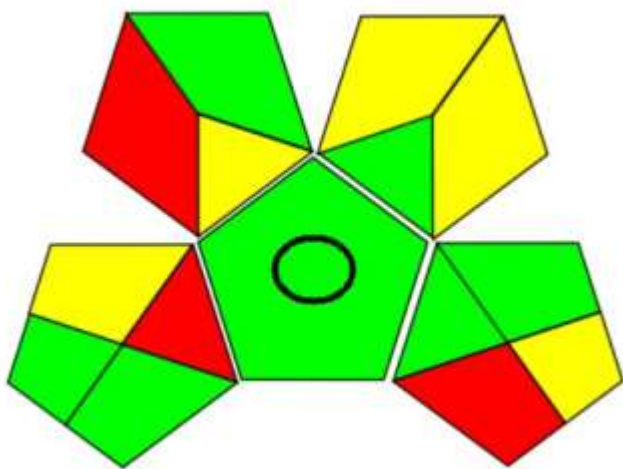
Figure 6: Assessment of greenness of the analytical method by GAPI metric.
