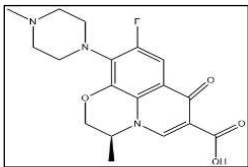
Figure 1: Chemical structure of LVF.
