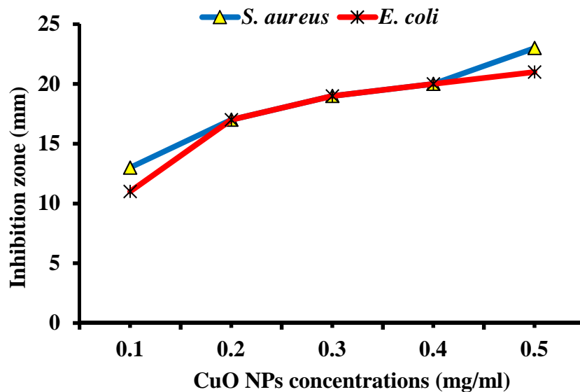
Fig (2): Inhibition zone of E. coli and S. aureus .
