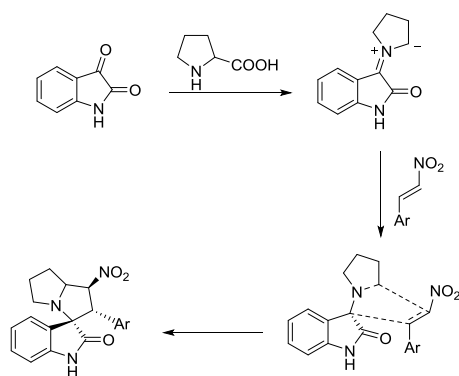
Scheme 2. Synthesis of spiro derivatives from isatin
