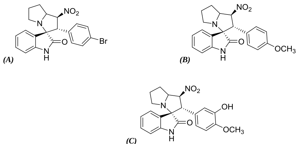
Scheme 1. Structure formula of spiro compounds (A,B C)
