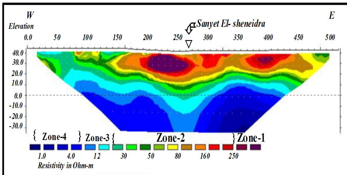
Fig. (12) 2- D resistivity imaging profile at Sanyet El-Sheneidra .
