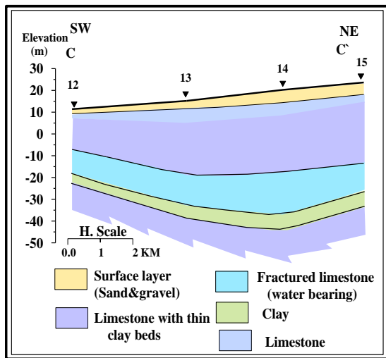
Fig. (8) Goelectrical cross section C-C'.
