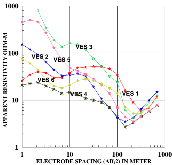
Figure (3 -a) Electrical sounding curves in the study area
