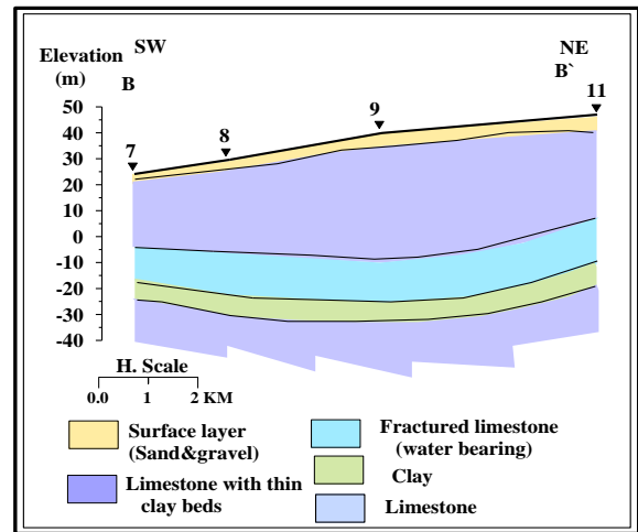
Fig. (7) Goelectrical cross section B-B'.
