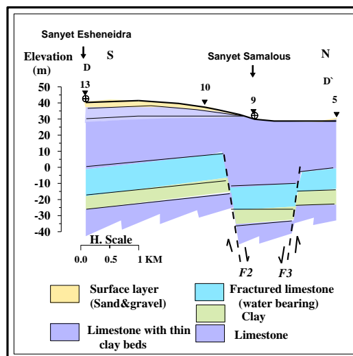
Fig. (10) Goelectrical cross section D-D'.
