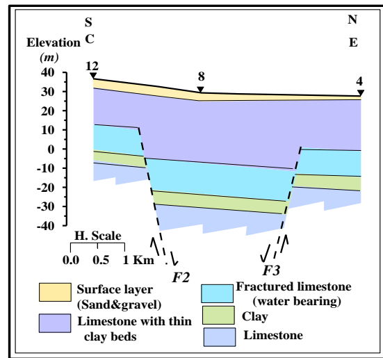
Fig. (9) Goelectrical cross section C-E.
