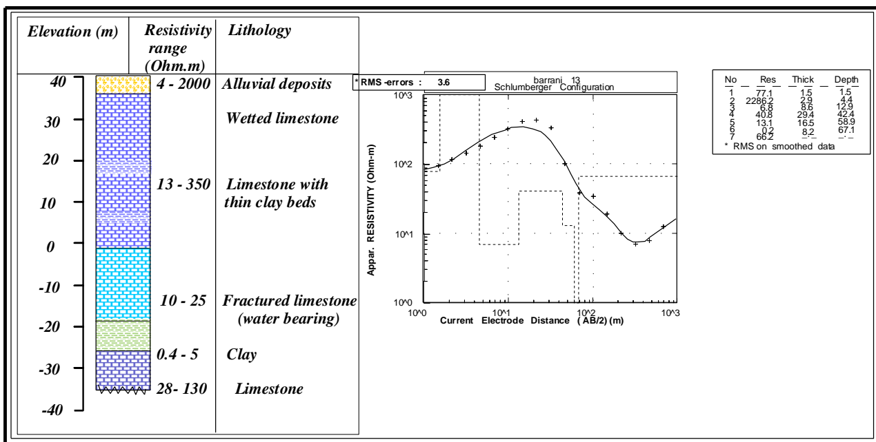
Figure (5) Range of resistivities and corresponding lithological data in the study area and the interpreted results of VES No.13 at Sanyet Esheneidra (Hand dug well)
