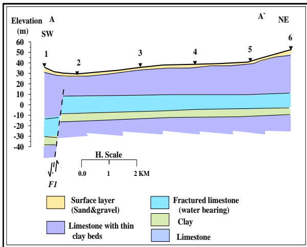
Fig. (6) Goelectrical cross section A-A'.
