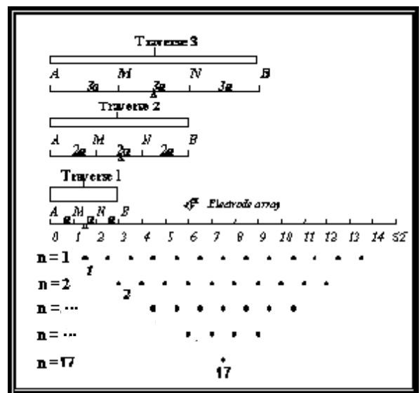
Figure (4) The measurement sequence for building up the electrical imaging section
