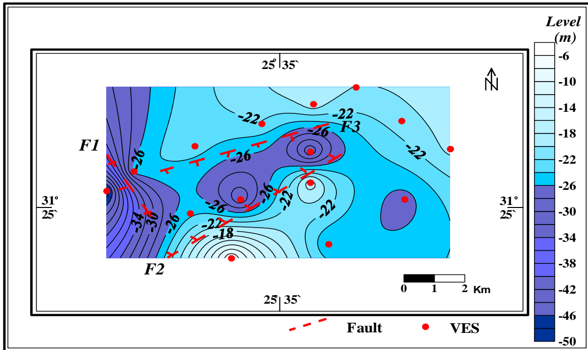
Fig. (11) Structural contour map of the upper surface of the last layer in the geoelectrical succession.
