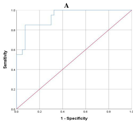
Figure 1: ROC curve showing performance of miRNA 1281-fold change in diagnosis of (A) proliferative diabetic retinopathy, (B) non-proliferative
