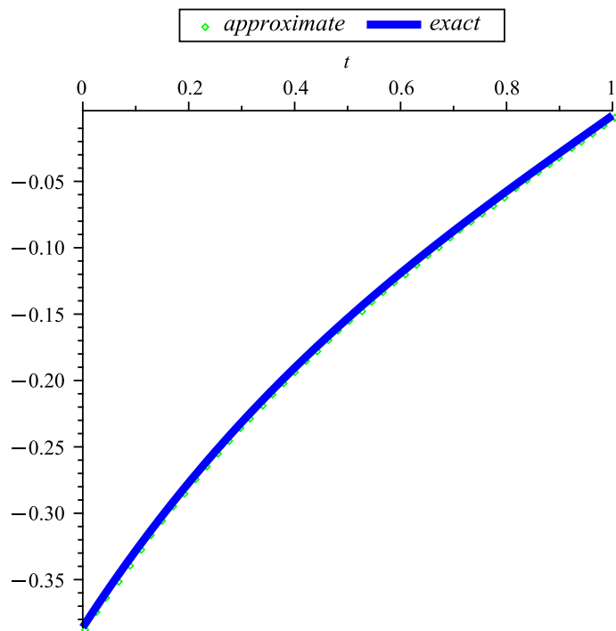
Fig. 4 The graphs of approximated and exact solution u(t) for Example 3.
