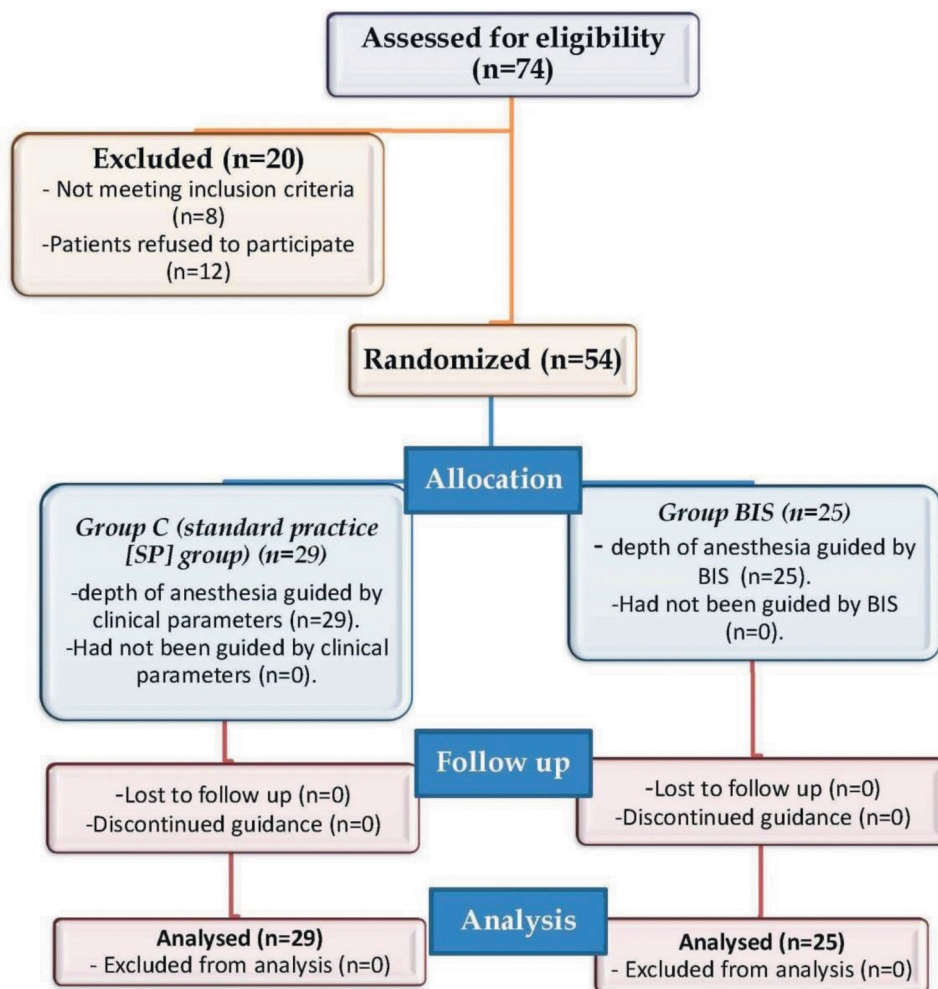
Figure 1. Concert flowchart.
