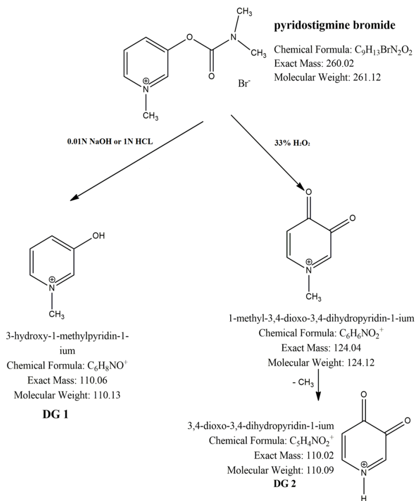
Fig. 1: Suggested pathway for the degradation of pyridostigmine bromide in 0.01N NaOH, 1N HCl and 33% H 2 O 2 .
