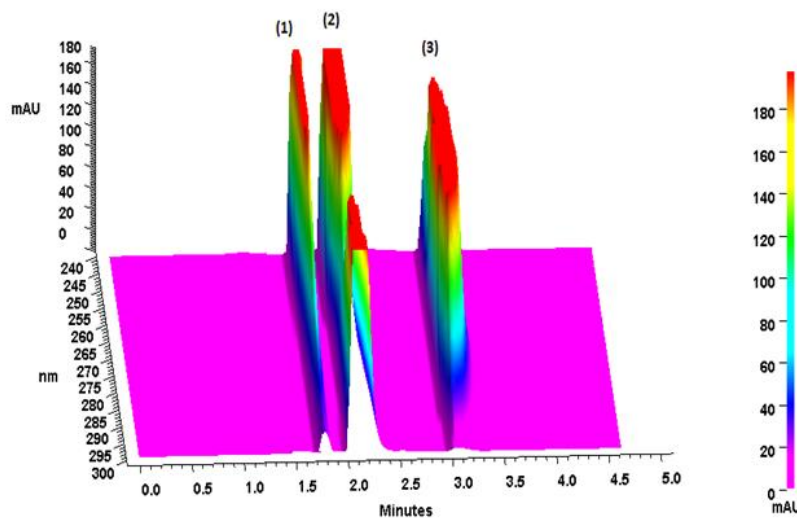
Fig. 6: DAD Spectrochromatogram of (1) DG2, (2) DG1 and (3) pyridostigmine bromide.
