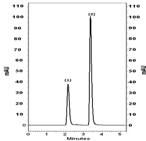
Fig. 3: HPLC chromatogram of pyridostigmine bromide in acidic media (1) [3hydroxy-1-methyl pyridine-1-ium] , (2) pyridostigmine bromide.
