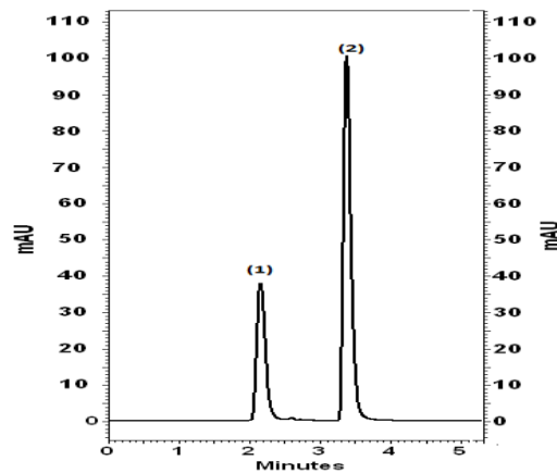
Fig. 4: HPLC chromatogram of pyridostigmine bromide in acidic media (1) [3hydroxy-1-methyl pyridine-1-ium] , (2) pyridostigmine bromide.
