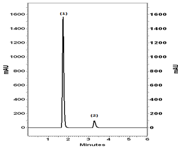
Fig. 5: HPLC chromatogram of pyridostigmine bromide in presence of 33% H 2 O 2 for 6 hours (1) [3, 4 -dioxo-3, 4-dihydropyridin-1-ium], (2) pyridostigmine bromide.
