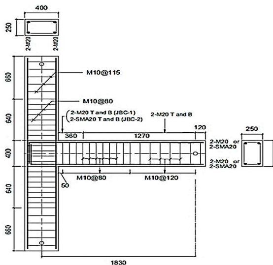
Fig. 4: Reinforcement Details of Specimens.
