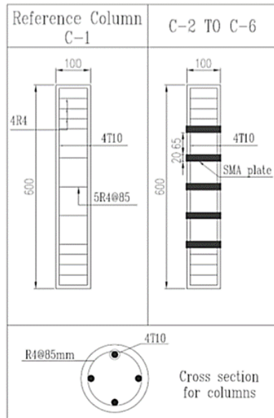
Fig. 9: Reinforcement Details of Specimens.
