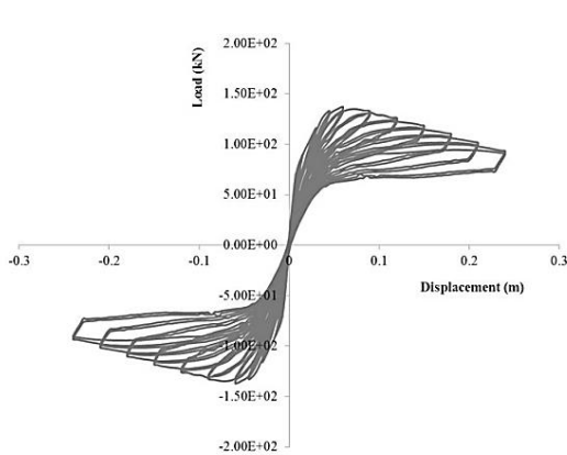
Fig. 7: Hysteresis curve of SMA-RC-Cu.
