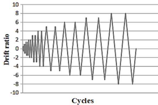
Fig. 7: Loading Protocol.
