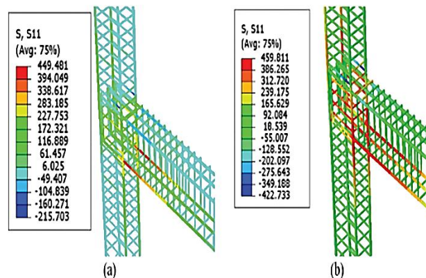
Fig. 5: Stresses of SMA Plates and Wire.
