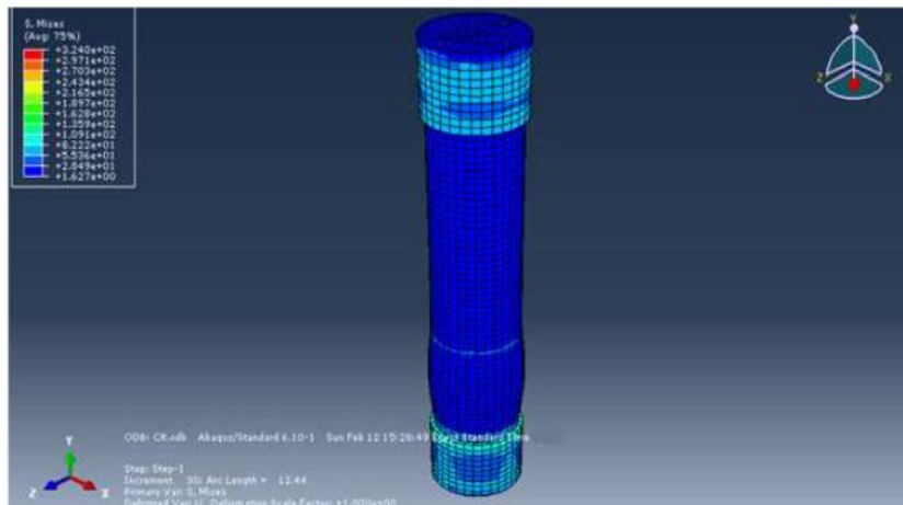
Fig. 10: Deformed Shape of Specimens.
