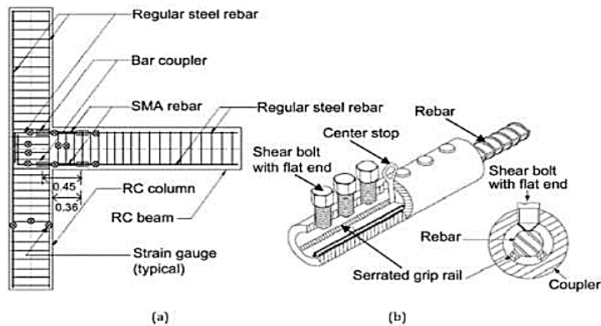
Fig. 3: Superelastic Ni-Ti SMA Bars for BCJ Details: (a) SMA and Steel bar Details; (b) Coupler.
