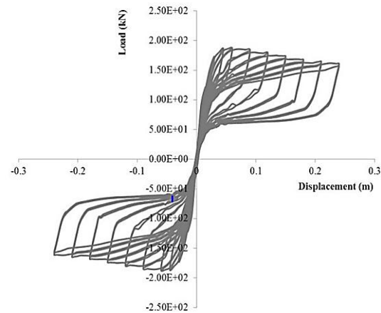
Fig. 8: Hysteresis curve of SMA-RC-Fe2.
