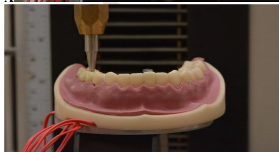
Figure 6. Application of load on center of fixed partial denture A, Vertical load. B, 30-degree oblique load.
