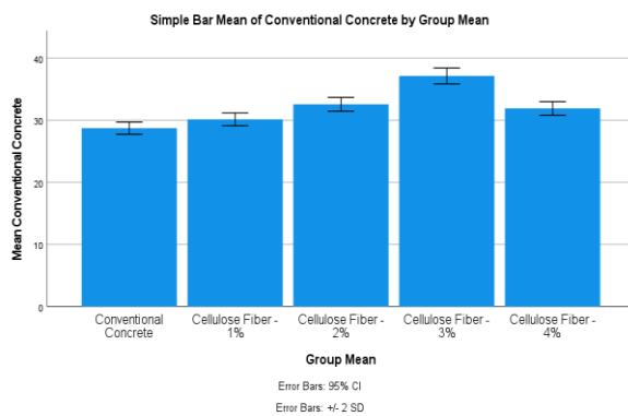
Figure 6: Comparison of Compressive Strength in N/mm^2 with cellulose fiber by various percentage. Derived chart was prepared by using SPSS Statistics version 27.
