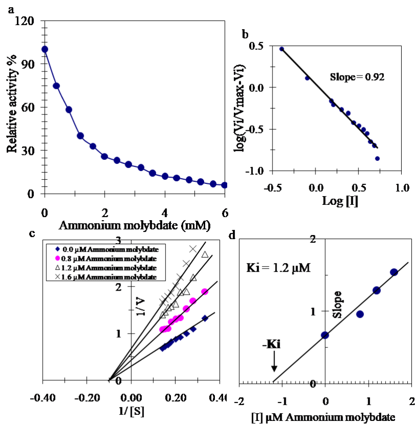
Fig. 5. (a) Inhibition of the purified BVACP by varying concentrations of ammonium molybdate. (b) Hill plot for inhibition of BVACP by varying concentrations of ammonium molybdate. (c) Lineweaver-Burk plots showing the type of inhibition of BVACP by ammonium molybdate. (d) Determination of the inhibition constant ( K_i ) value for the inhibition of BVACP by ammonium molybdate.
