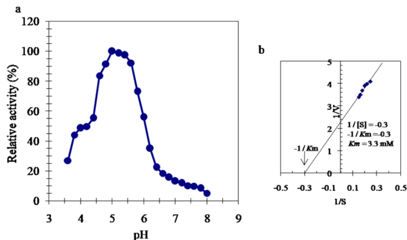
Fig. 3. (a) pH effect on the purified BVACP using 20 \text{ mmol L}^{-1} Na-acetate buffer (pH 3.6 to 5.6) and Na-phosphate buffer (pH 5.7 to 8.0). (b) Lineweaver-Burk plot relating the reciprocal of the reaction velocity of the purified BVACP to p -NPP concentration in mM.
