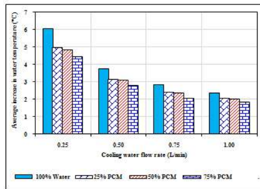
Fig. 8: Average increase in the cooling water outlet temperature.
