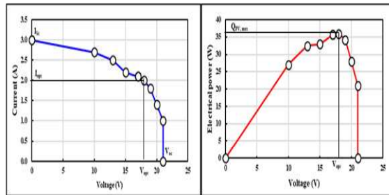
Fig.5: Characteristic curves for the PV cell.
