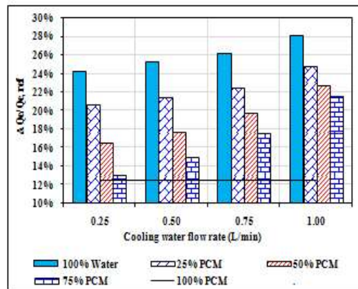
Fig. 11: The average percentage increase in the PV electrical power.
