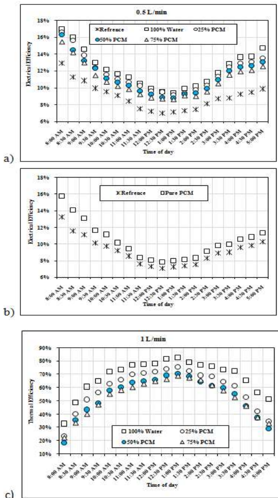
Fig. 9: PV electrical and thermal efficiencies.
