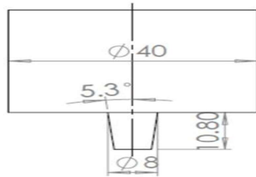
Fig. 2 Schematic illustration of the tool used in the present study dimensions in mm
