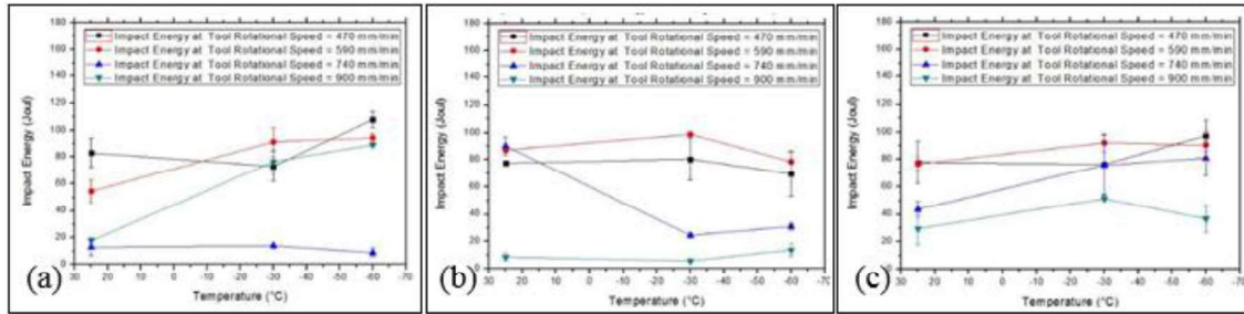
Fig. 9. Effect of Temperature on Impact Energy at Different Welding Transverse Speed:
