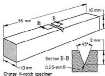
Fig. 3 Charpy V-notch dimensions According to ASTM E23.
