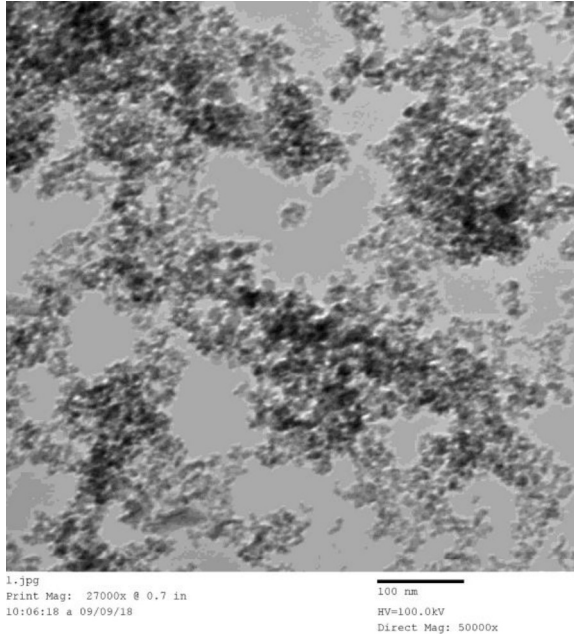
Fig. 4a. TEM photograph of \text{Al}_2\text{O}_3 nanoparticles
