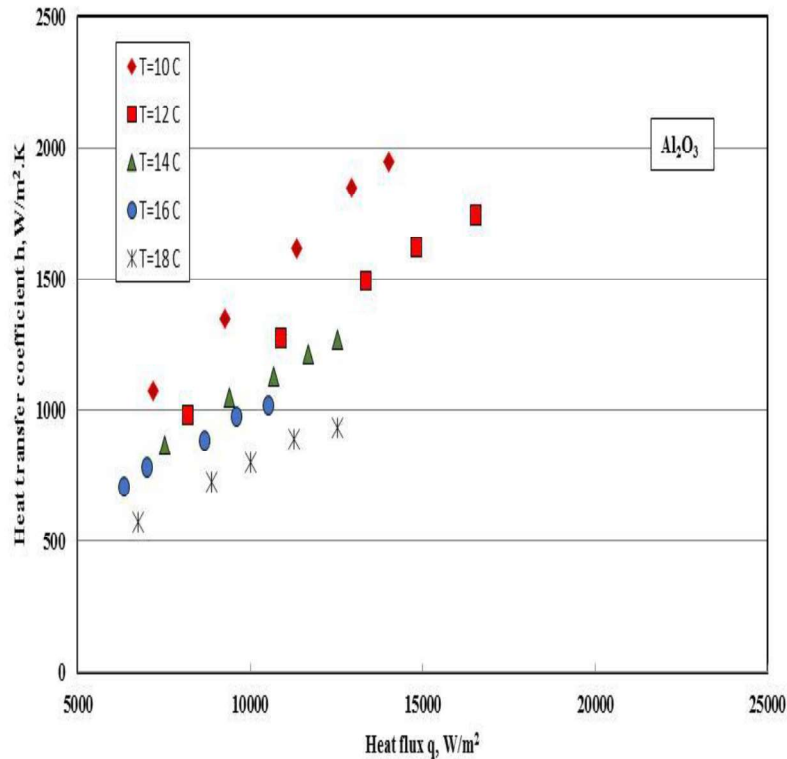
Fig. 9: Variation of evaporating htc with heat flux for different inlet water temperature for \text{Al}_2\text{O}_3 -R134a based nanofluid of void fraction of 0.50%.
