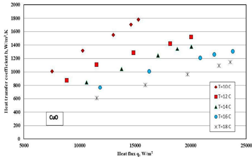
Fig. 10: Variation of evaporating htc with heat flux for different inlet water temperature for \text{CuO} -R134a based nanofluid of void fraction of 0.09%.
