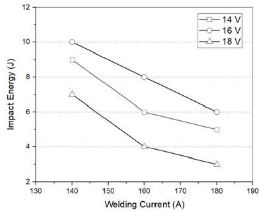
Fig (9). Variation of the impact energy with welding current for samples MIG technique using different welding voltages.
