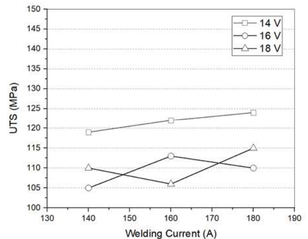
Fig (11). Variation of UTS with welding current for samples MIG technique using different welding voltages.
