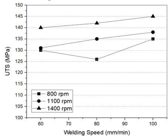
Fig (10). Variation of UTS with welding speed for samples FSW using different tool rotational speeds.
