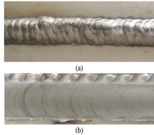
Fig (4). Photographs of the (a) MIG and (b) FSW welded plates.
