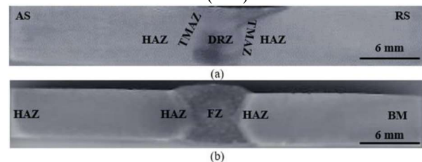
Fig (5). Photographs showing the macrostructure of the (a) FSW sample welded using 1100 rpm and 80 mm/min; and (b) MIG sample welded using 16 V and 160 A.
