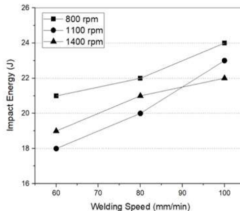
Fig (8). Variation of the impact energy with welding speed for samples FSW using different tool rotational speeds.
