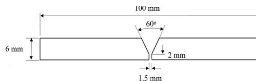
Fig (2). V-butt joint configuration of MIG welding samples.
