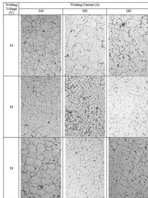
Fig (7). Microstructure at the center of FZ for AA6061-O samples MIG welded using different voltages and currents ( \times 100 ).
