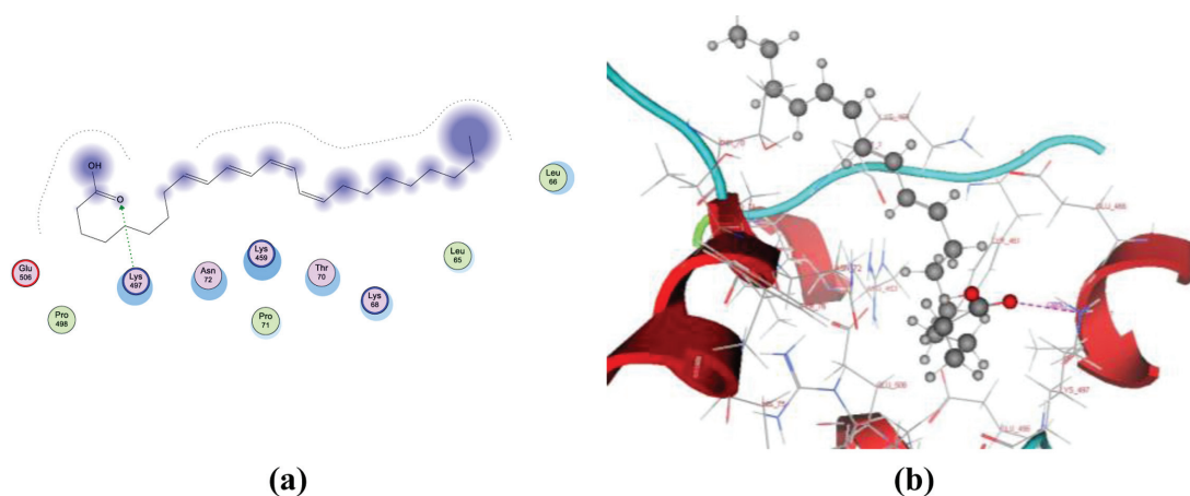
Molecular docking of compound 1 (a) two-dimensional; binding modes and (b) three-dimensional; mapping surface of compound 1 with COX-2 with Score Energy= -19.2858 kcal/mol.
