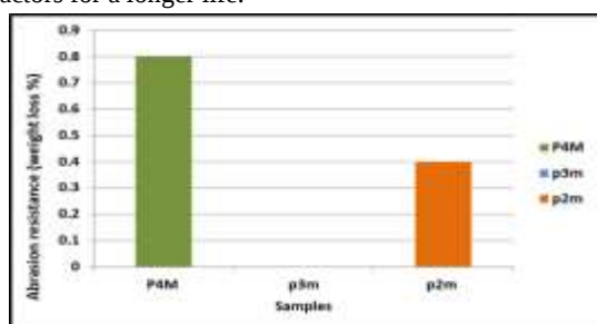
Figure 10. Abrasion resistance (weight loss%) for the best three samples in properties
