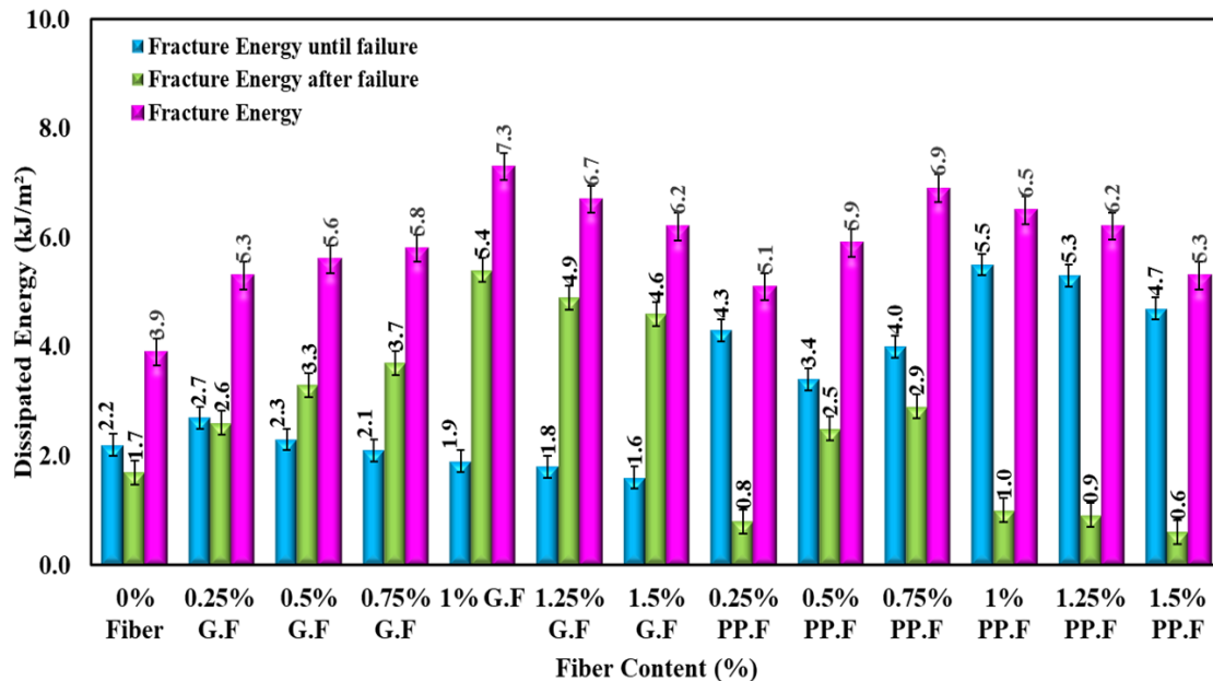
Fig.17. Effect of the addition of different amounts of polypropylene and glass fibers on fracture energy parameters of bituminous mixtures.
