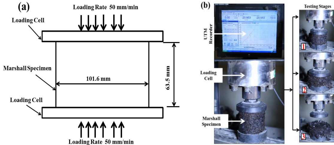
Fig.7. Compressive strength test data (a) Loading applied mechanism and (b) Testing set-up and deformation stages.
