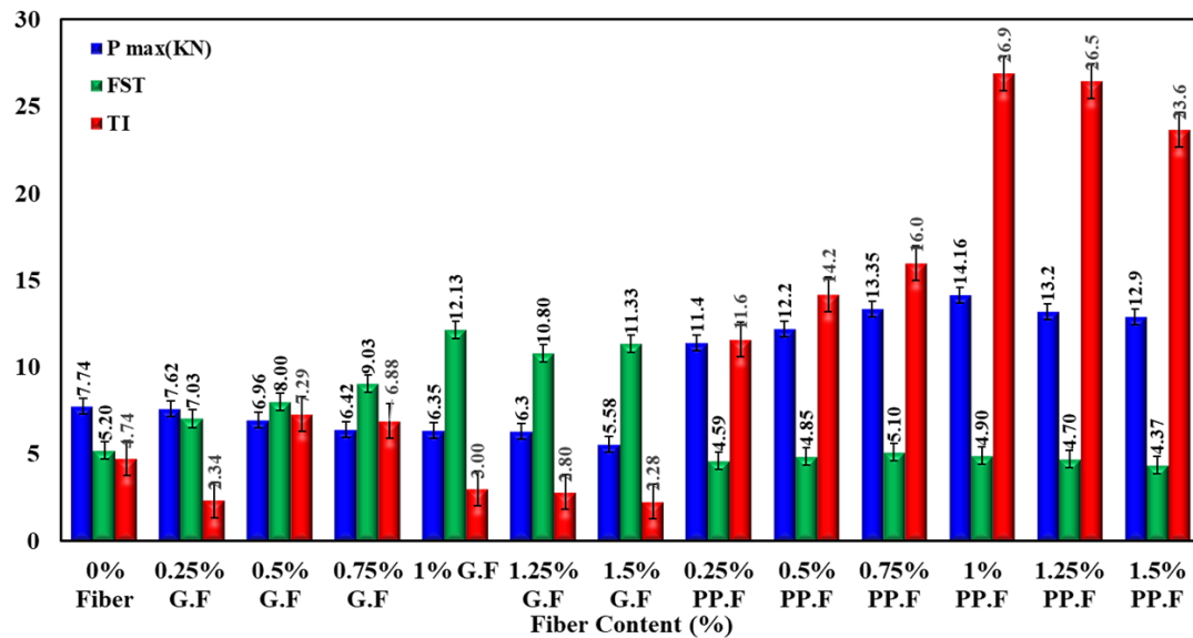
Fig.18. Effect of the addition of different amounts of polypropylene and glass fibers on fracture resistance indexes of Pmax, FST and TI of bituminous mixtures.
