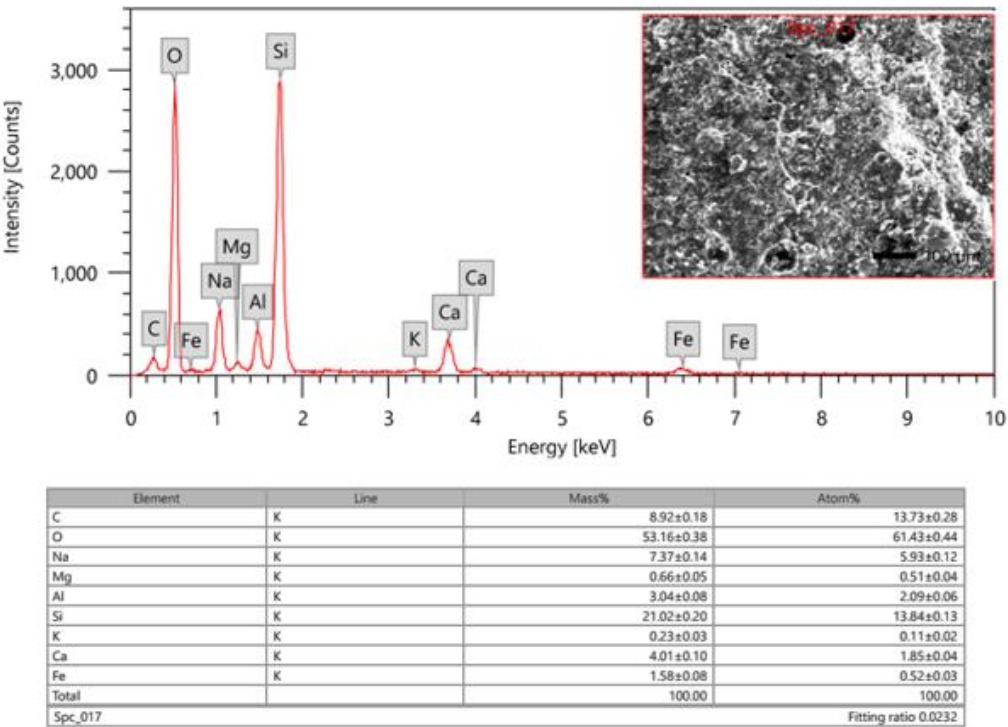
Figure 6. EDX analysis of GPM
