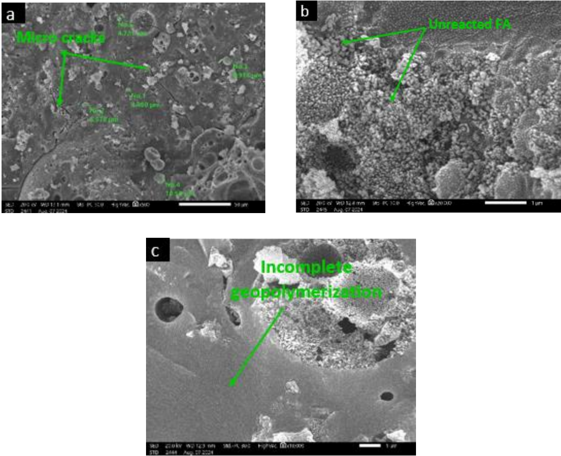
Figure 5. SEM analysis of GPM
