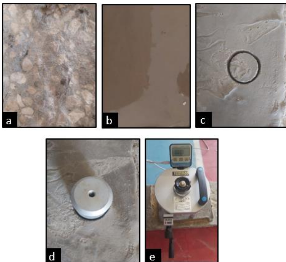
Figure 2. Experimental sequences of pull-off test of GPM overlay
