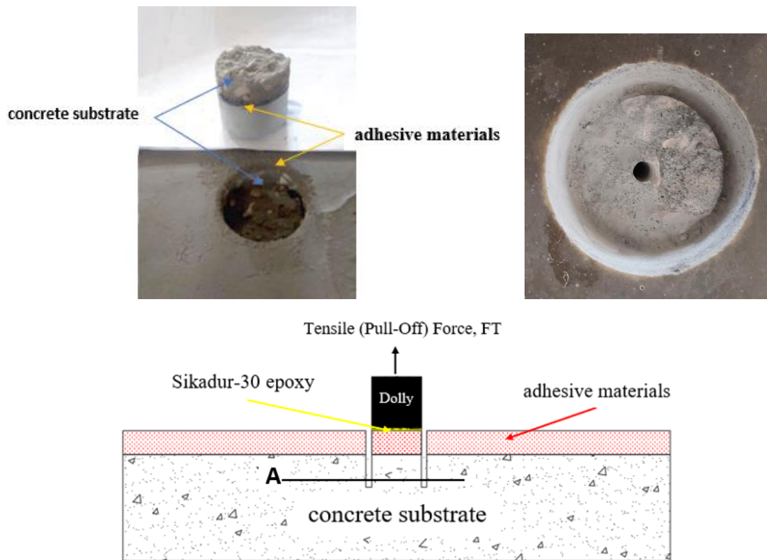
Figure 3. Failure modes of the pull-off test for of the specimens.
