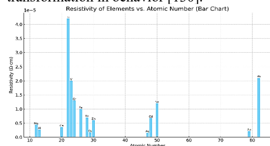
Figure 1. Resistivity vs Atomic Number of metallic elements
