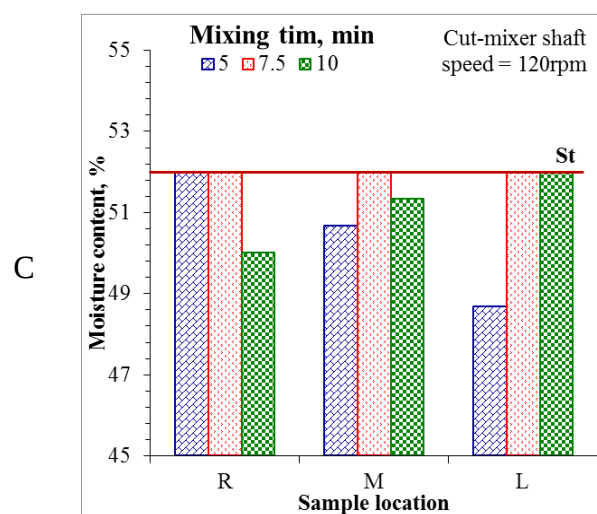
Fig 3: Mixture moisture content via samples location at different mixing time.
