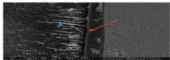
Figure (3) group (A1B1): SEM photomicrographs of nanoleakage at adhesive interface of universal single bond doped with zinc chloride using etch and rinse adhesive technique.
