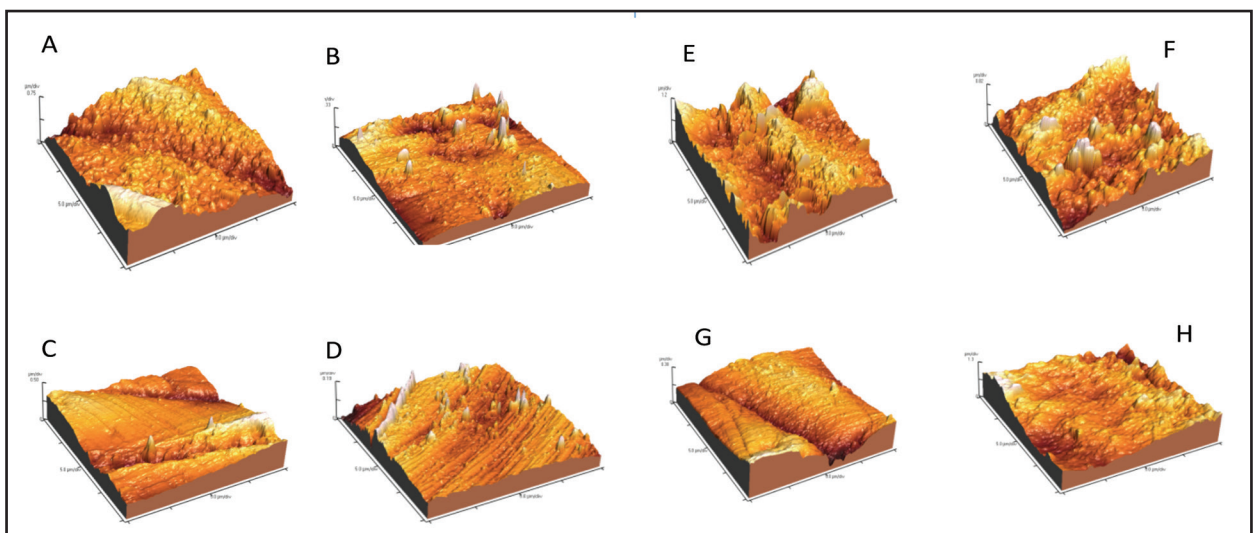
Figure (4) Topographic 3D image for cubic zirconia; a) control specimen b) control after LTD c) laser specimen ,d) laser specimen after LTD Topographic 3D image for tetragonal zirconia; e) control specimen,f) control after LTD ,g) laser specimen, h) laser specimen after LTD
