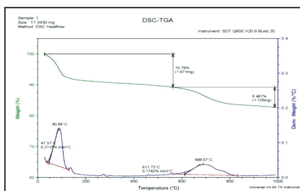
Figure (3): Thermogravimetric traces of MMT-AgNPS hybrid
