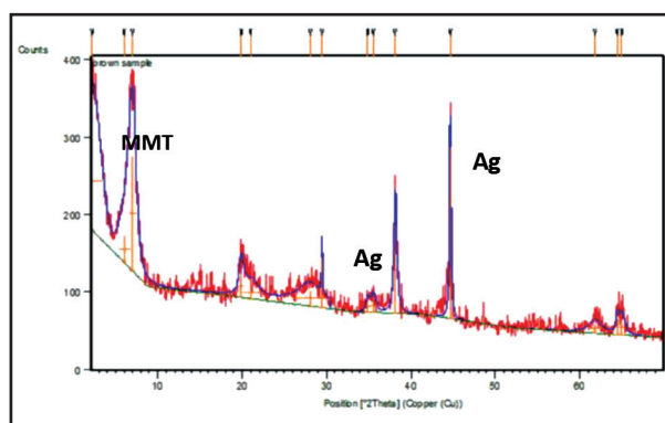
Figure (2): XRD pattern of MMT loaded by AgNPs
