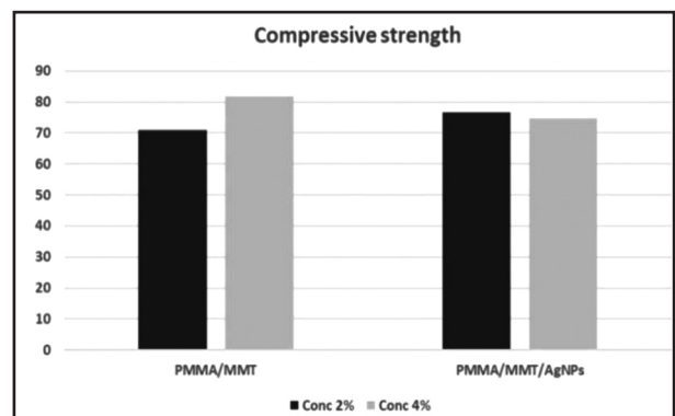
Figure (4): Compressive strength values of different groups with different concentrations
