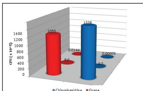
Figure (4) 3D cylindrical chart comparing mean of CFU of pre, post 48 hr and post 1 week for chlorohexidine group and grape seed extract group.
