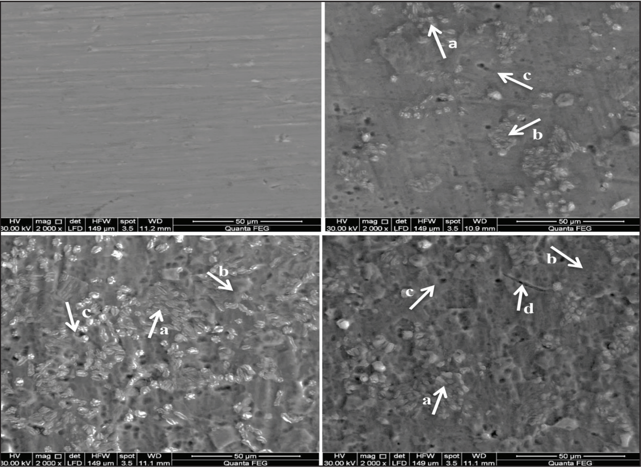
Figure (7): SE micrographs of the control group and the anodized coated groups where:The (a) arrow pointed to the silica crystals, the (b) arrow pointed to the titania islands, the (c) arrow pointed to the porosities, the (d) arrow pointed to the developed cracks.
