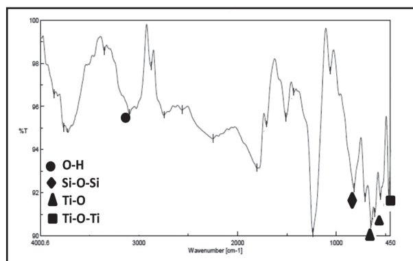
Figure (4): AT-FTIR spectrum of the anodized coated samples showing the stretching bands of O-H, Ti-O, Ti-O-Ti and SiO 2
