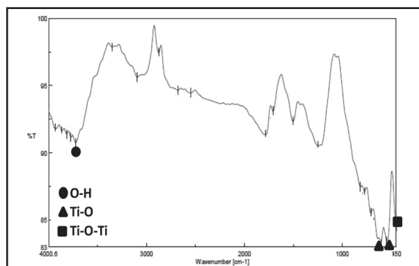
Figure (3): AT-FTIR spectrum of the control group showing the stretching bands of O-H, Ti-O, Ti-O-Ti
