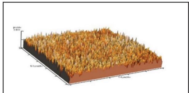
Figure(2) 3-D microphotograph of glass ionomer with coat before brushing with mean surface roughness (Ra) = 8.71nm.
