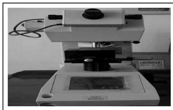
Fig. (1) Vickers Microhardness Tester. A: Eye Piece lens, B: Working table, C: Loading force hand wheel, D: Digital screen
