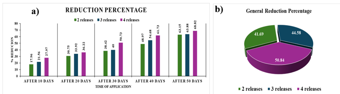
Fig. 4: Comparative Reduction of Cabbage Achieved by Varying Trichogramma evanescens Release Numbers (2, 3, 4) Over Time (10, 20, 30, 40, and 50 Days).
