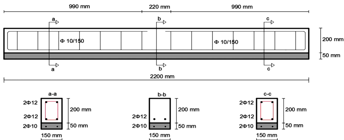
Figure 7. Strengthening using UHPFRC [135].
