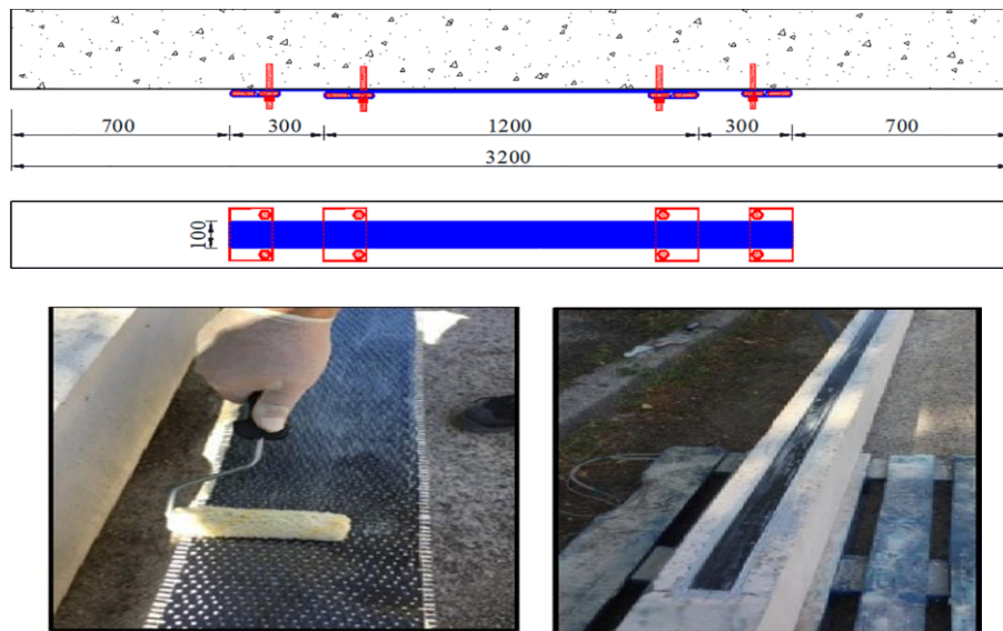
a) EB-CFRP plates or sheets [113].
