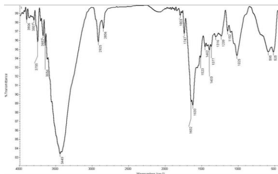
Figure 5. Fourier transform infrared (FTIR) spectrum of AgNPs synthesized by Fusarium oxysporum showing different functional groups responsible to stabilize or cap AgNPs.
