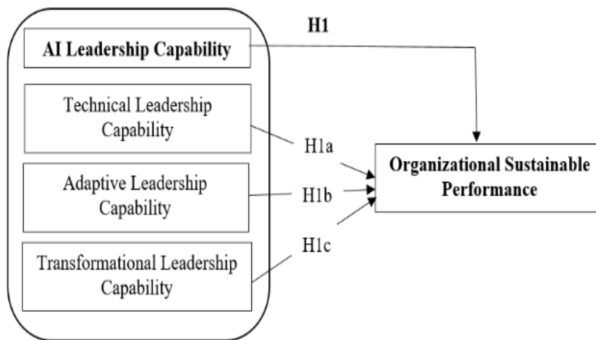
Figure 1: Theoretical Framework
