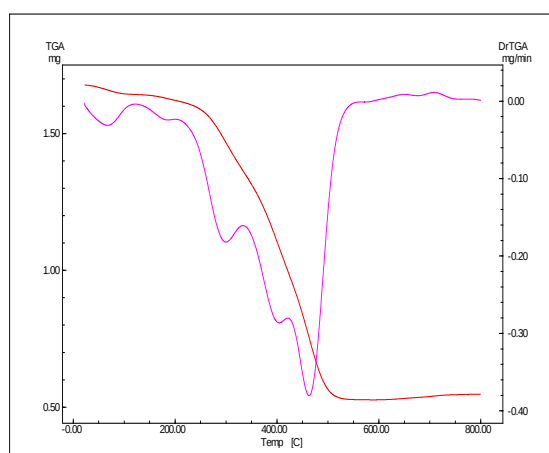
Zn(II)-complex
