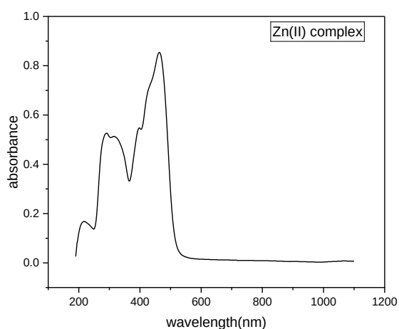
Zn(II)-complex
