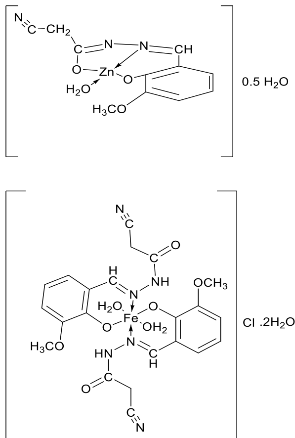
Fig (1): The structures of [\text{Zn}(\text{L})(\text{H}_2\text{O})]\cdot 0.5\text{H}_2\text{O} and [\text{Fe}(\text{HL})_2(\text{H}_2\text{O})_2]\cdot \text{Cl} \cdot 2\text{H}_2\text{O} complex
