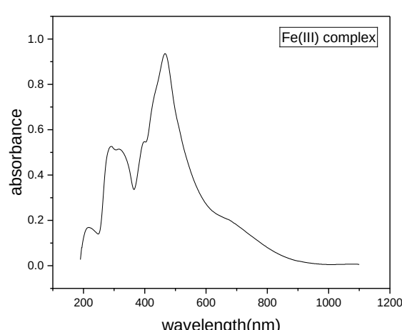
Fe(III)-complex
