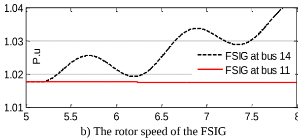
Fig. 11 The response of the FSIG when connected to bus 11 or 14 for the considered disturbance
