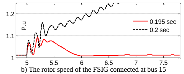
Fig. 8 Response of the FSIG connected at bus 15 when subjected to a three-phase short circuit at the PCC.
