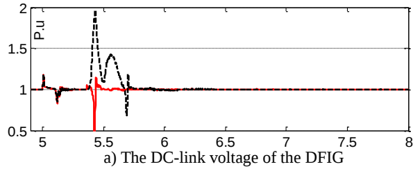
Fig. 6 Response of the DFIG during grid disturbance (1- The DFIG is equipped with crowbar protection circuit 2- The DFIG is equipped with chopper protection circuit)
