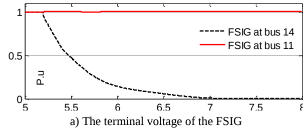
Fig. 10. FSIG performance for a short circuit fault at the PCC point for different penetration ratio
