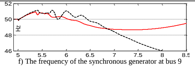
Fig. 7 Effect of short circuit duration on the power system stability considering the DFIG at bus 15
