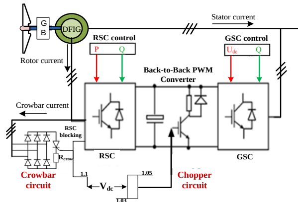
Fig. 2 Configuration of double fed induction generator-based wind turbine [3]
