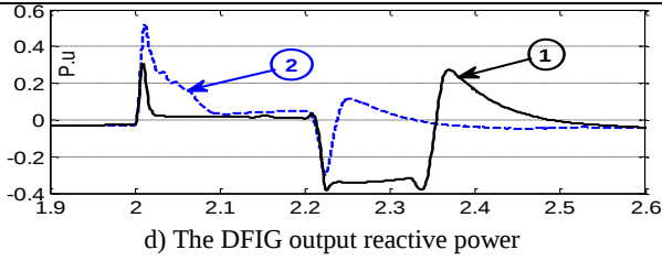
Fig. 6 Response of the DFIG during grid disturbance (1- The DFIG is equipped with crowbar protection circuit 2- The DFIG is equipped with chopper protection circuit)
