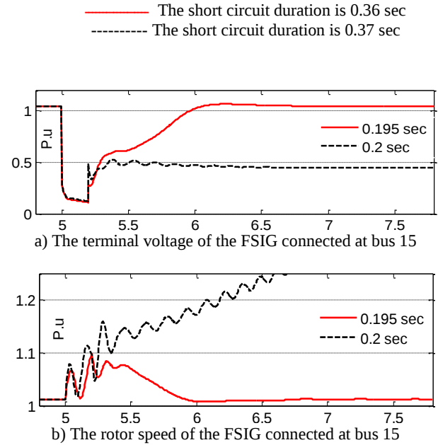
Fig. 8 Response of the FSIG connected at bus 15 when subjected to a three-phase short circuit at the PCC.
