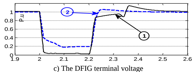
c) The DFIG terminal voltage
