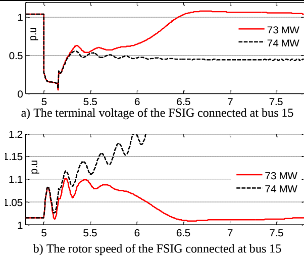
Fig. 10. FSIG performance for a short circuit fault at the PCC point for different penetration ratio
