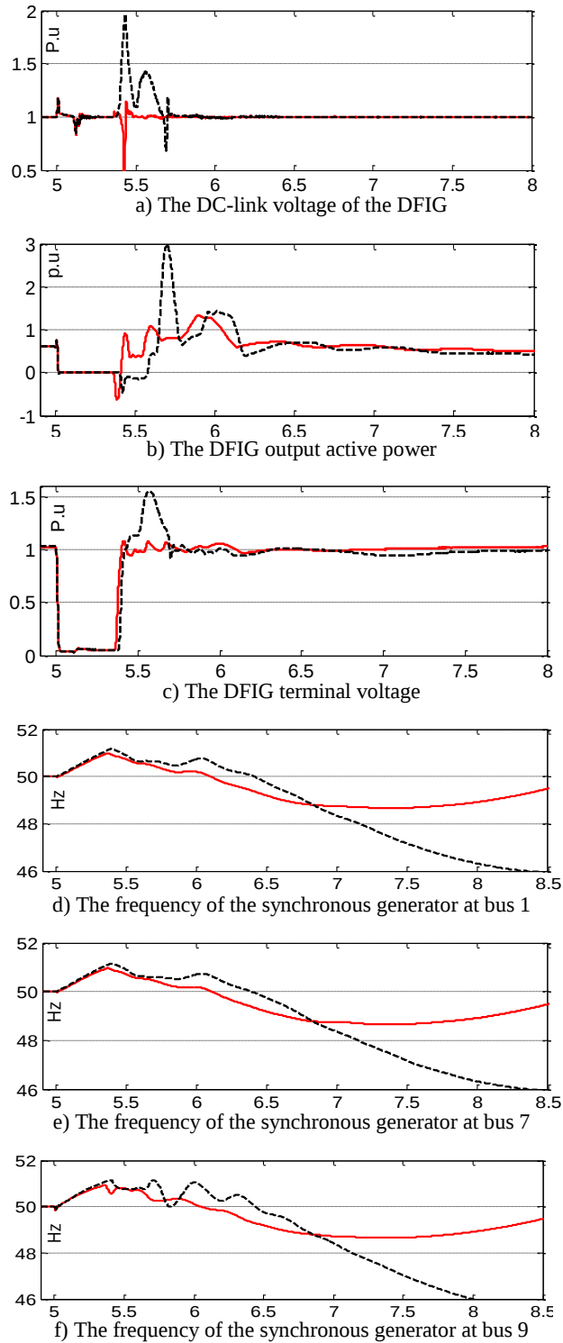
Fig. 6 Response of the DFIG during grid disturbance (1- The DFIG is equipped with crowbar protection circuit 2- The DFIG is equipped with chopper protection circuit)
