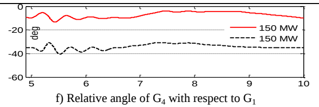
Fig. 9 The power system response for a three-phase short circuit at the PCC of the DFIG wind farm with different penetration levels
