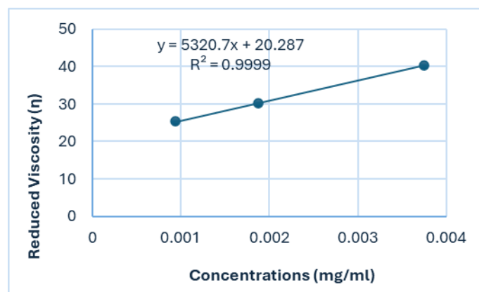
Fig 3. Reduced viscosity versus concentration of EPS68.
