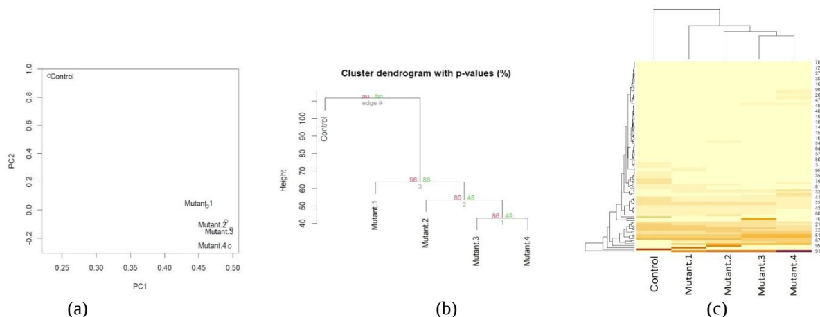
Fig. (1). Multivariate statistical analysis of the phytochemical constituents of leaves of L. leucocephala mutagenized seedlings. (a) Principal component analysis (PCA) of four mutants (Mutant 1, Mutant 2, Mutant 3, and Mutant 4) and the control of L. leucocephala . A PCA was based on the correlation matrix of phytochemical composition in control, mutant 1, mutant 2, mutant 3, and mutant 4. The first and second principal components accounted for 66.8% and 17.8% of variation, respectively; (b) A consensus tree of the relationships among control, mutant 1, mutant 2, mutant 3, and mutant 4 of L. leucocephala . Pvcust package in R was used to cluster these traits according to the Euclidean distance matrix. The numbers at the forks were the percentages of approximately unbiased (AU; in red) p-values and bootstrap probabilities (BP, in green) estimated from 1000 bootstrapping samples; (c) A heatmap showing cluster groups in both phytochemical composition and different mutants of L. leucocephala (control, mutant 1, mutant 2, mutant 3, and mutant 4). The numbers on the right side represent the codes for 106 phytochemical components within five solvents that showed a mixed pattern.
