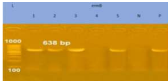
Fig. 5. Gel electrophoresis of PCR amplification products for the ermB gene in Clostridium perfringens isolates. Lanes 1,2 ,3 &5 showing positive amplification of the ermB gene, associated with resistance to macrolide, lincosamide, and streptogramin B antibiotics. Lane P: positive control; Lane N: negative control; Lane L: 1 kb DNA ladder.
