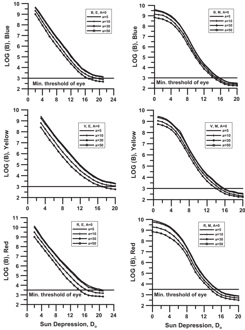
Fig. 5 The relation between \log B expressed in S_{10} ( B , V , R ) units with the sun's depression ( D_0 ) at the site, for the evening ( E ) and morning ( M ) sky twilight at azimuth A = 0^\circ and at altitudes a = 5^\circ, 10^\circ, 30^\circ, 50^\circ , above the horizon.
