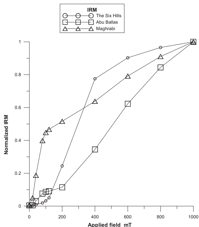
Fig. 3 Examples of IRM acquisition curves for the studied formations.
