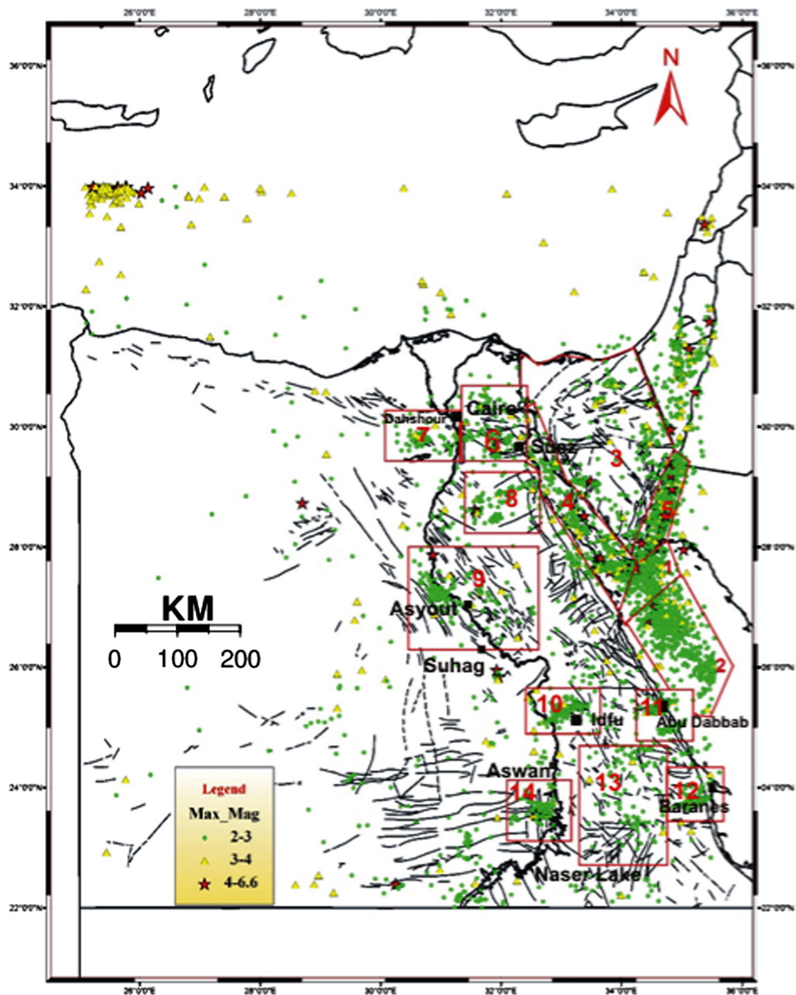
Figure 1 Distribution of the earthquake epicenters during the period from 2004 to 2011 and the different seismic source regions in Egypt are represented by numbers.
