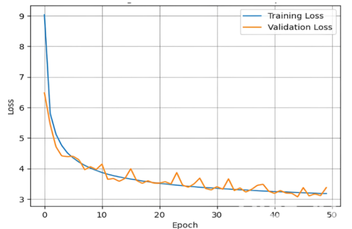
Fig. 6 Training and Validation loss in ANN model with epoch
