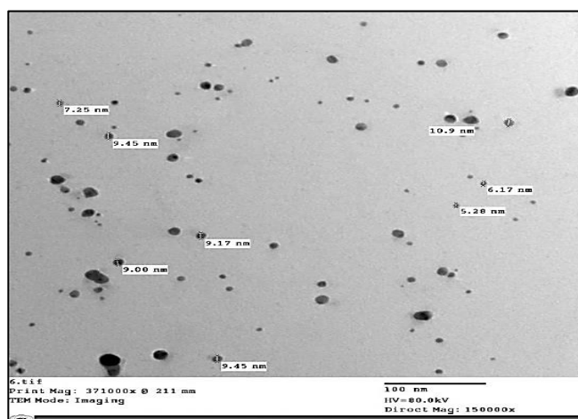
Figure 2. Transmission electron microscope (TEM) image of silver nanoparticles
