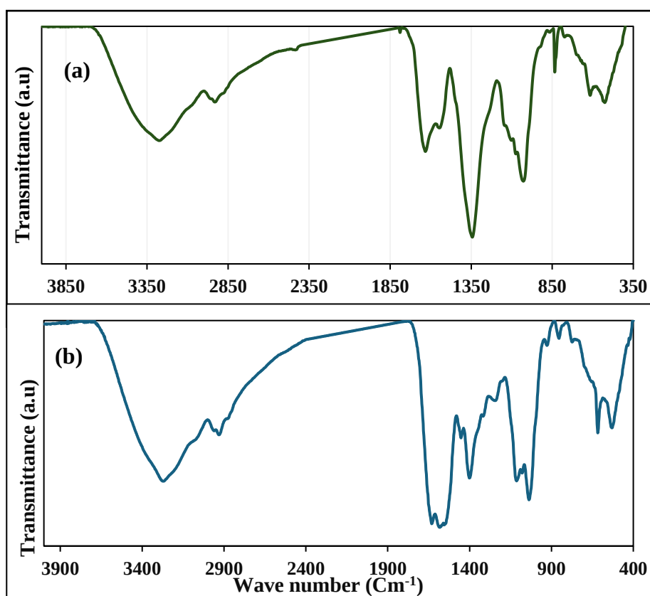
Figure 3. (a) The FT-IR spectrum of SP-Ag-NPs produced using the crude aqueous extract from Spirulina platensis , and (b) the FT-IR spectrum of the crude aqueous extract of Spirulina platensis .
