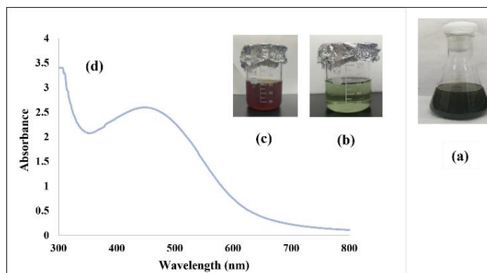
Figure 1. (a) Spirulina platensis aqueous extract (b) \text{AgNO}_3 (c) SP-AgNPs (d) UV.VIS spectrum of SP-Ag-NPs produced by Spirulina platensis
