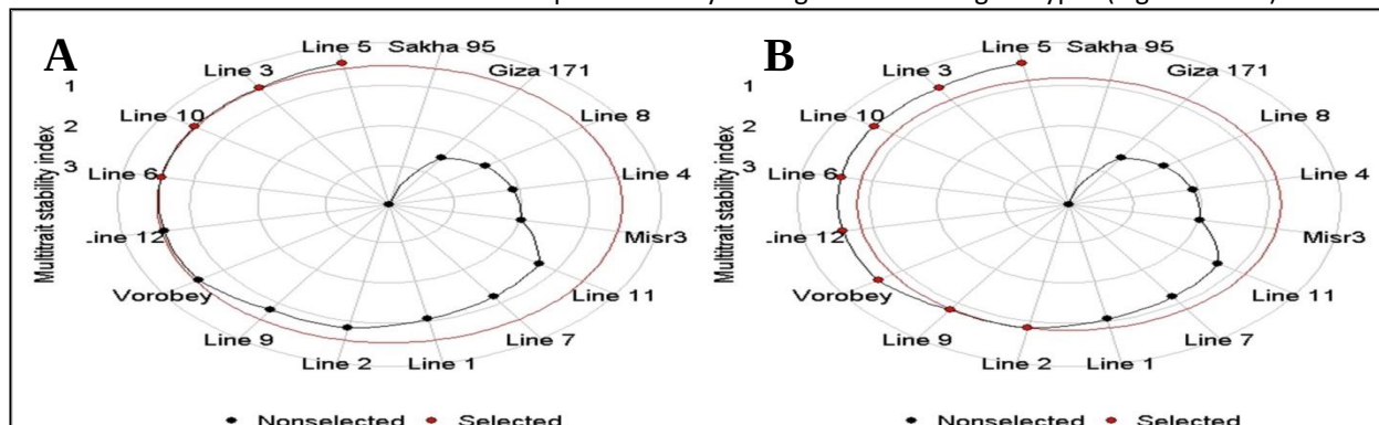
Fig. 3. Genotypes are ranked based on (MTSI) across GY and specific agronomic traits (Third Scenario). Red dots represent the selected best genotypes, with the central red circle indicating cutoff points for selection pressures of 25% (A) and 50% (B).
